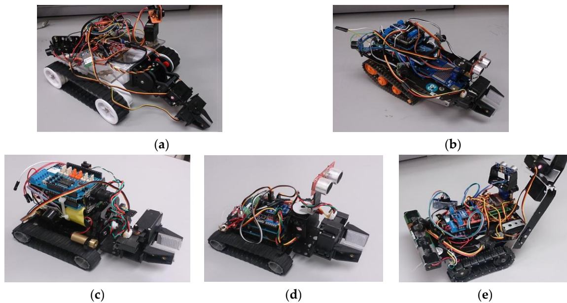
Figure 6. The heterogeneous swarm robots showing different configurations. (a) Robot R_1 with 4-Dof arm; (b) Robot R_2 with 1-Dof arm ; (c) Robot R_3 with onboard blackfin camera; (d) Robot R_4 showing two kinds of sensors at the front; (e) Robot R_5 with 3-Dof arm and a camera.
