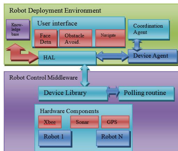
Figure 2. Software architecture.
